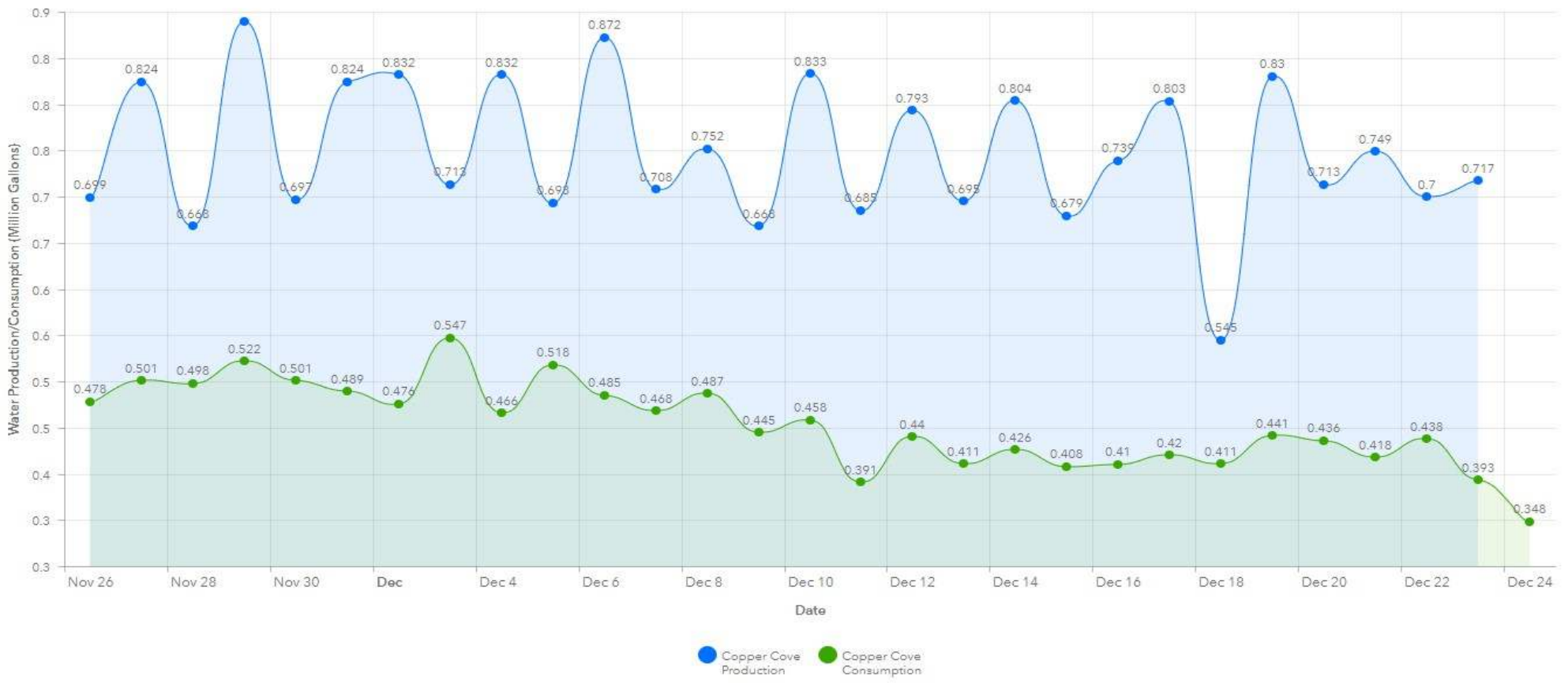
Copper Cove Water Production/Consumption
