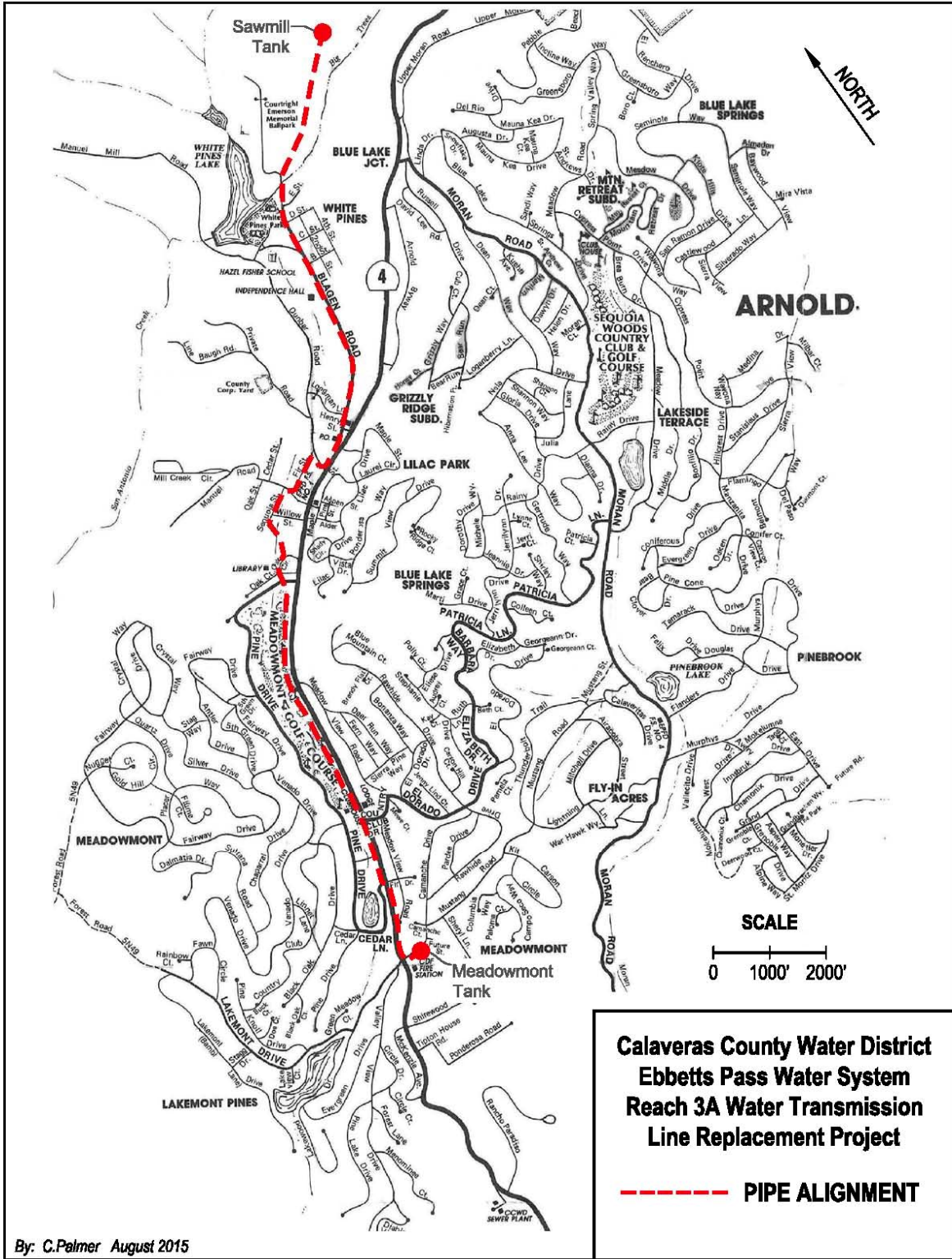
FIGURE 1: REACH 3A PROJECT ALIGNMENT
